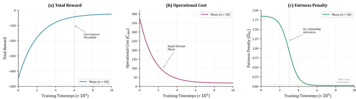
Note. Solid lines denote mean values and shaded bands denote 95% confidence intervals. Panel (a) reports the total reward over training steps. Panel (b) reports the operational cost component of the objective, which captures staffing shortfalls and overtime penalties. Panel (c) reports the counterfactual fairness penalty measured as the Kullback-Leibler divergence between policy distributions for factual and counterfactual states. The curves show rapid early feasibility learning, stabilization of the reward trajectory after approximately 600,000 steps, and a later decline in fairness loss after annealing of the counterfactual regularization weight ( \lambda_{CF} ) is annealed.
