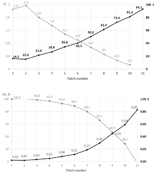
» Figure 7: Lightness (L) and optical density (D) values are linear along the visually uniform step wedge printed in equal data intervals from PDF/X file (upper) in contrast to the printed tone value TV or luminance Y (lower)
