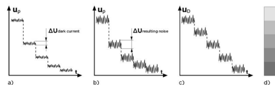
» Figure 5: Forms of reflectance U_p and density U_D signals for visually uniform tone scale (d): at the sensor output (a) and at the end of a channel without (b) and with the use (c) of logarithm transform
